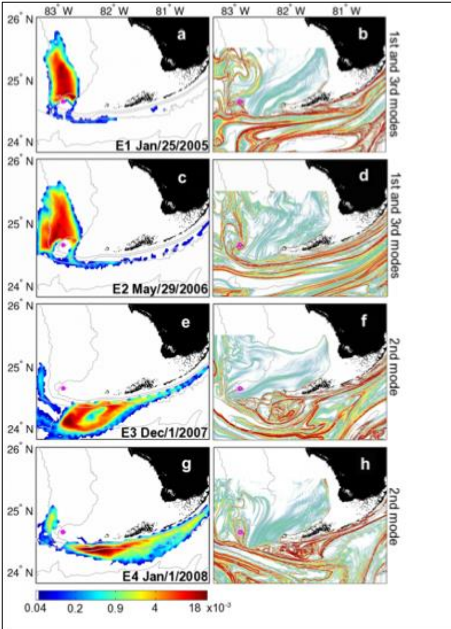
Figure 12. Larval pathways and flow characteristics during four settlement events. Left column ( a,c,e,g ): probability density function (PDF) of larval trajectories calculated over 12 days before the end of the pelagic larval duration. Right column ( b,d,f,h ): attracting Lagrangian Coherent Structures (LCSs) obtained from Finite-Time Lyapunov Exponents (FTLE). The four settlement events, namely E1 = Jan/25/2005, E2 = May/29/2006, E3 = Dec/01/2007, and E4 = Jan/01/2008, correspond to high settlement pulses identified in figure 4. (FTLE).
