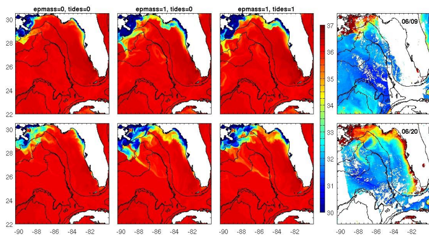
Figure 1: (Left 3 panels) Sea surface salinity from three 1/50^\circ Gulf of Mexico simulations (zooms) with different attributes for the Mississippi River (MR) parameterization and the tides: no MR momentum flux, no tides; MR momentum flux, no tides; MR Momentum flux, tides. (Right panel) observed ocean color, for comparison. Two different dates are shown: June 9, 2014 (top), June 20, 2014 (bottom). The black lines indicate the 200, 2000, and 3000 m isobaths.
