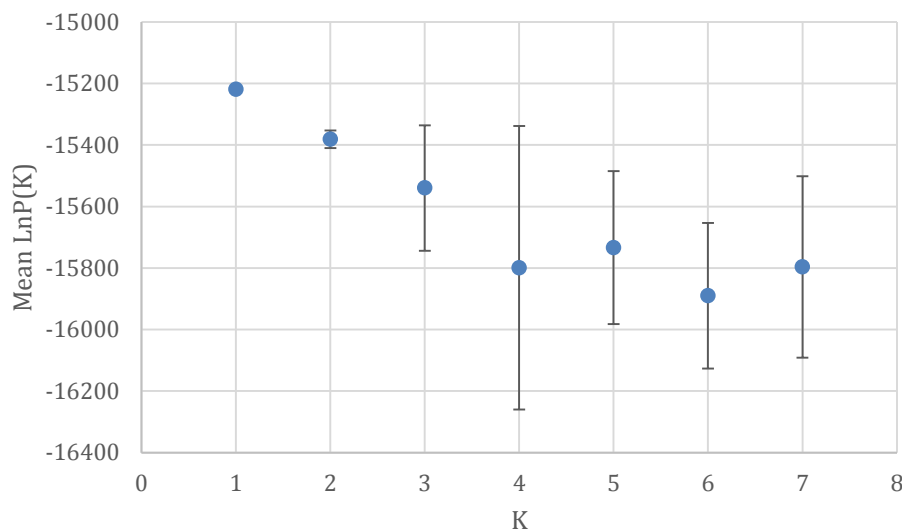
Figure 3. Structure output of the mean estimated Ln Probability of Data: LnP(D) ( \pm std. dev.) vs. cluster number ( K ) ( K = 1-7 ) across five independent runs (100 000 burn-in, 100 000 MCMC iterations) assuming the locprior model and correlated allele frequencies.
