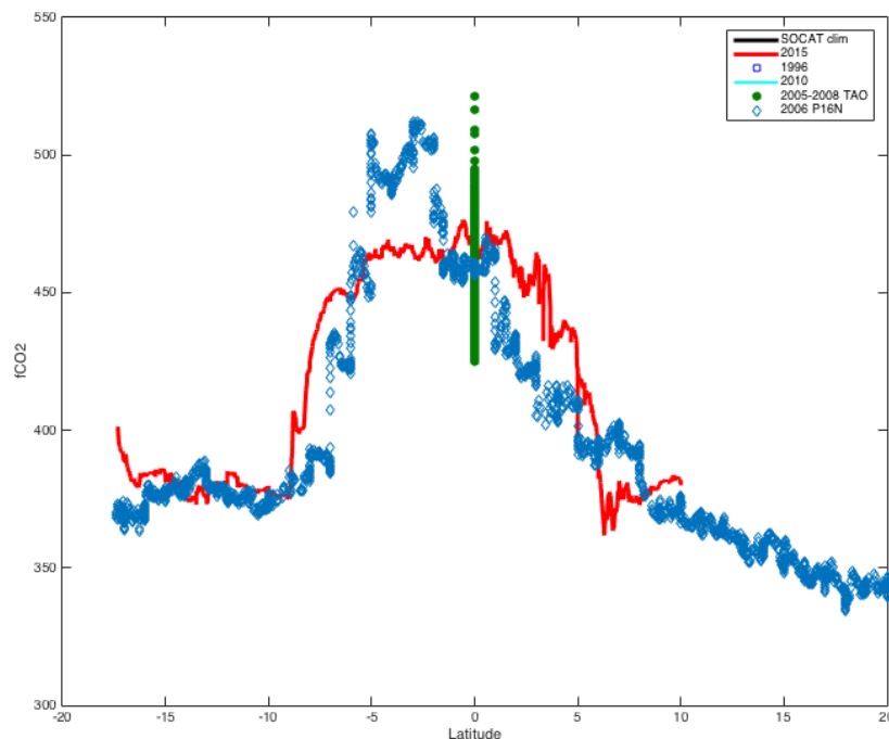
Figure 1 caption: Surface water CO 2 levels during P16N (red line) compared to previous occupations and mooring data at 0°N, 155°W (green line). The lower peak values and higher SST (not shown) near the equator indicate the onset of an El Niño during April/May 2015 (plot courtesy of S. Siedlecki).
