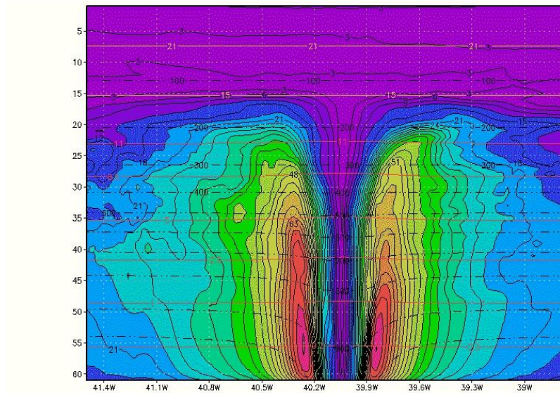
Figure 5: Vertical XZ slice of horizontal wind field for idealized TC at y = 22.39 degrees; same time and domain as for Figure 3. Contours every 3 \text{ m s}^{-1} . Vertical axes gives model level, with level 1 being the model top. Also shown are isolines of constant pressure (hPa) by dot-dash black lines, and geopotential height (km) by solid colored isolines. The pressure increment is 100 hPa except for a 50 hPa increment between the lowest two isobaric surfaces with the lowest being at 950 hPa. A maximum horizontal wind of \sim 75 \text{ m s}^{-1} (146 kt) occurs in both the western and eastern portions of the eyewall at \sim 300 m elevation.
