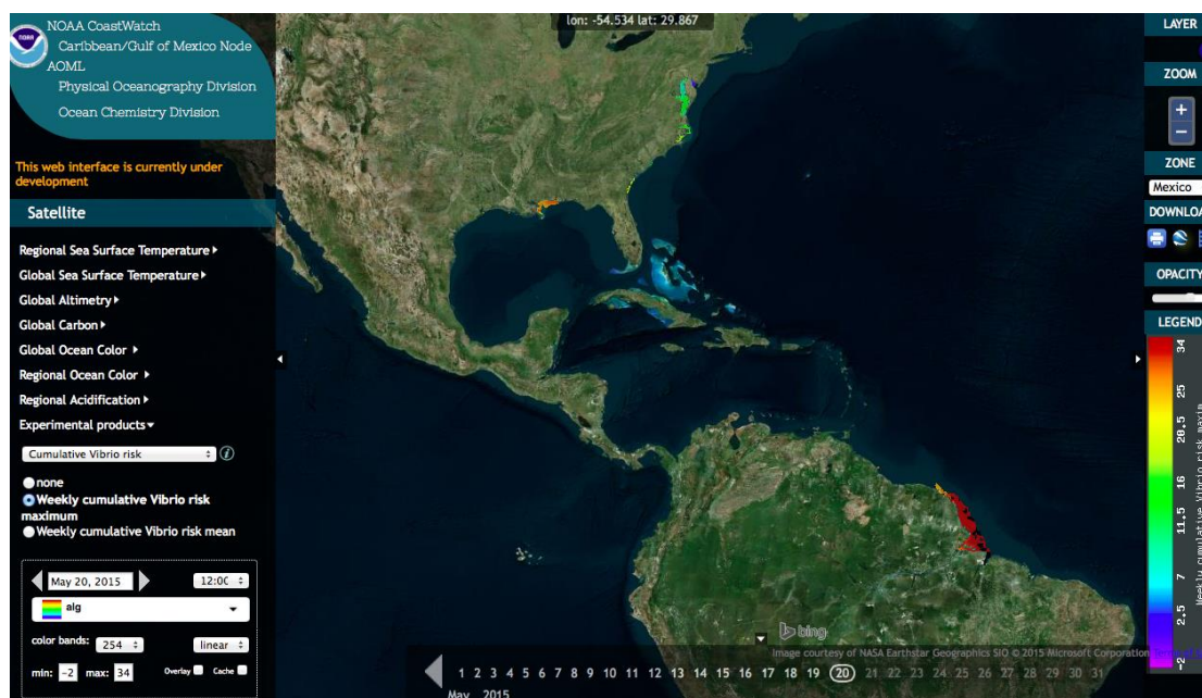
Figure 2: Weekly cumulative vibrio risk maximum displayed using the online viewer. Regions in Chesapeake Bay, Mississippi delta, and Brazil show significant risk. These fields are largely determined by sea surface temperature and sea surface salinity.
