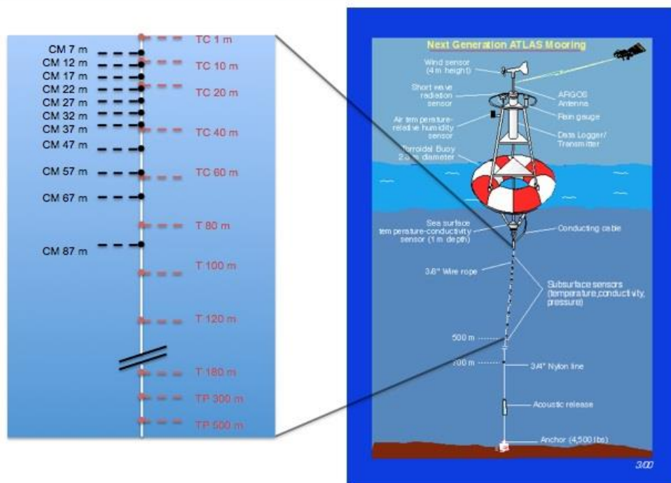
Figure 2: Schematic of the TACOS current meter instruments deployed on the 4N, 23W PNE mooring on January 23, 2015.
