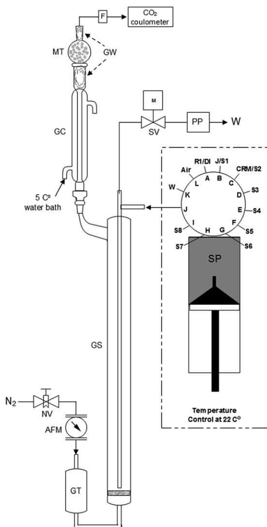
Figure 6. A schematic diagram of the multi-sample automated naturalwater analyzer (MANA). Acronyms: NV, needle valve; AFM, air-flow meter; GT, glass trap; GS, glass stripper; GC, glass condenser; MT, moisture trap; GW, glass wool; F, PTFE 0.2 mmfilter; SV, pinching valve; PP,
