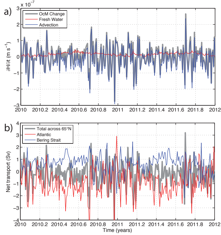
Figure 24. (a) The time change of the Arctic OcM (gray), the net transport across 65^\circ\text{N} scaled by the ocean area north of this latitude (blue), and fresh water fluxes (red); (b) net transport in Sverdrups ( 1 \text{ Sv} = 10^6 \text{ m}^3 \text{ s}^{-1} ): total across 65^\circ\text{N} (gray), across 65^\circ\text{N} in the Atlantic Ocean (red), and through the Bering Strait (blue).
