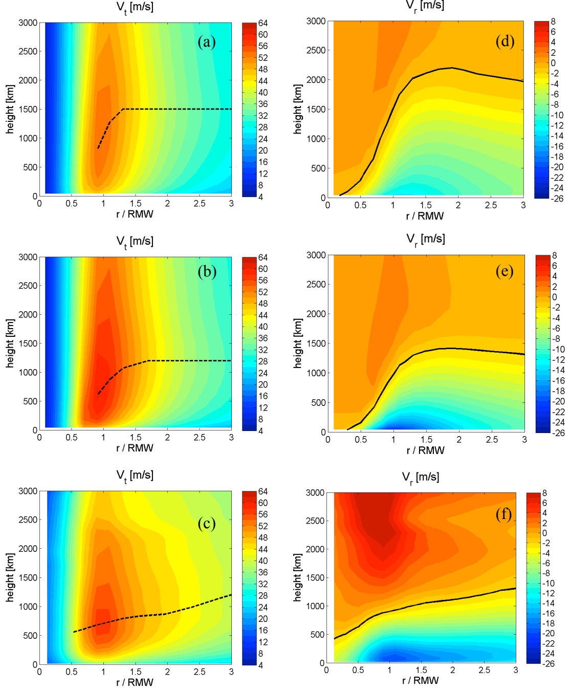
Figure 11: Plots of tangential wind (left) and radial wind (right) as a function of r/RMW and height. The upper panels are for PBL11, the middle panels are for PBL12, and the lower panels are for sonde composites from Zhang et al. (2011a). The dashed line represents the height of the maximum tangential wind speed and the solid line represents the inflow layer depth.
