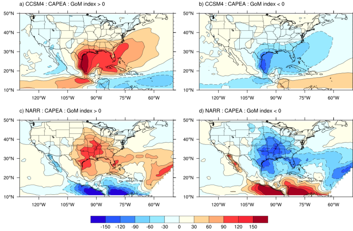
Figure 7: CAPE anomaly composite maps, associated with warm (left) and cold (right) SST anomaly in the Gulf of Mexico, in the CCSM4 (upper) and NARR (bottom). Composites are made from MJJ mean for the period 1982-2010. Unit of CAPE is J/kg.
