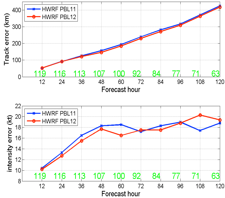
Figure 8: Absolute errors of track (upper panel) and intensity (lower panel) forecasts of the two sets of HWRP simulations of 4 hurricanes listed in Table 1.
