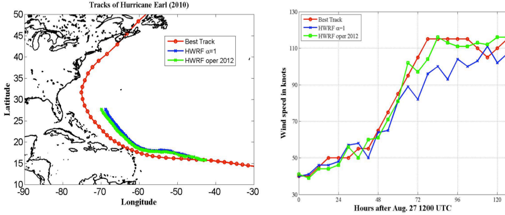
Figure 5: Intensity forecast of Hurricane Earl (2010) simulated using the 2012 version HWRf model with initialization at 12Z on August 27 using two different PBL physics, one following the 2012-version HWRf setup and the other following the 2011-version HWRf setup (see text for details).
