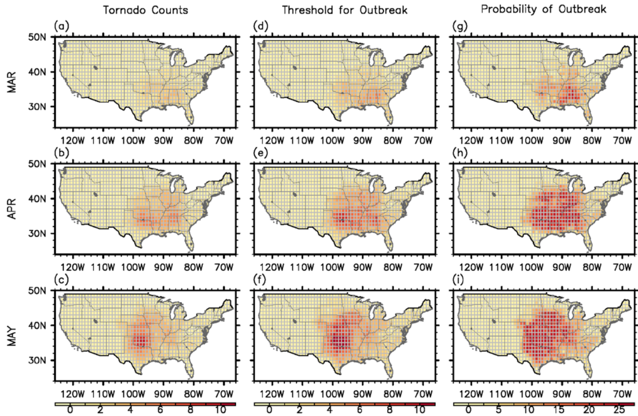
Figure 2. (Left panels) The climatological number of tornadoes within 200 km radius, (Mid panels) the threshold for outbreak and (Right panels) the probability (%) of US regional tornado outbreaks for March, April and May, obtained by using the four steps described above.
