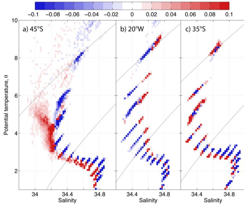
Figure 2: Modeled mean transport in Sv across three sections as a function of \theta -S, evaluated in a \Delta\theta - \Delta S bin of 0.2^\circ\text{C} - 0.02 . Positive values denoting northward or westward transport into the South Atlantic. The two isopycnals ( \sigma_2 of 35.80 and 36.62 \text{ kg m}^{-3} ) represent the upper and lower most layer of AAIW in model.
