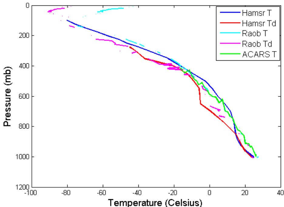
Figure 9: ACARS, rawinsonde and HAMSRS temperature and dewpoint from soundings taken at 0Z on Sept. 4, 2013 near Barbados, the approximate initial location of TC Gabrielle.
