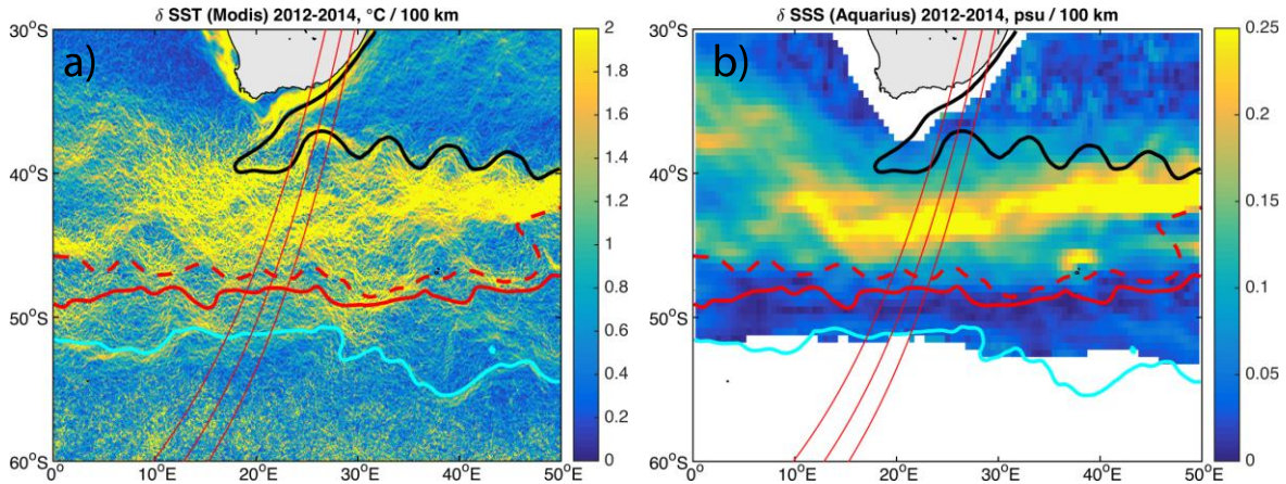
Figure 2. The horizontal absolute gradients of (a) SST from Modis (°C/100 km) and (b) SSS from Aquarius (psu/100 km, gridded product). The AR (black), SAF-N (dashed red), SAF (red), and PF (cyan) as identified in Figure 1 are shown.
