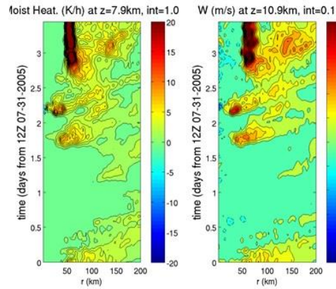
Figure 2: Structure changes in nature run (NRH1) before RI: a) surface to 8km (red) and 5km (black) tilt, along with the maximum azimuthal-mean tangential wind at z = 2\text{km} , which shows the large increase in intensity after 06Z August 3; b) Hovmoller diagrams of azimuthal-mean most heating and vertical velocity at z = 7.9 and 10.9\text{ km} , respectively. The azimuthal mean shows the contributions of two large convective bursts (which are in fact highly localized) before the eyewall forms.
