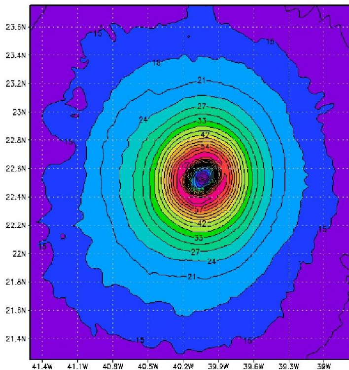
Figure 3: Surface wind field for idealized TC at 126hrs simulation, domain D03 (dx=dy=0.02780 ; mean resolution of 3.0 km). Contours every 3 ms -1 . Maximum wind = 64.3 ms -1 \approx 125 kt (144 mph). Mean radius of maximum wind = 18.6 km. Minimum eye wind = 4.4 ms -1 . NS wind gradient along southern inner eyewall = 5.4 ms -1 km -1 . Storm location 0.75 degrees S and 0.75 degrees E of point of initialization (net motion of 110 km towards SE).
