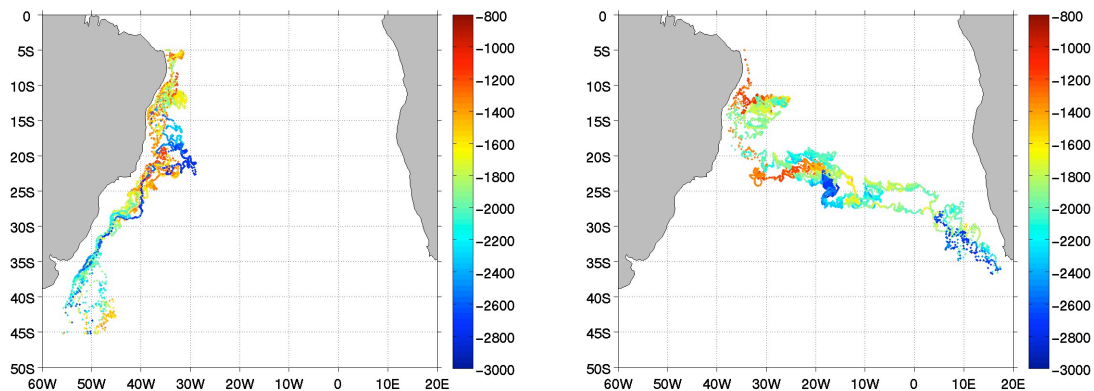
Figure 2. Examples of the two main pathways for the NADW derived from synthetic floats launched along 5°S between 1000 and 3500 m depth in the OFES model. The left panel shows examples of trajectories of 71% of the synthetic floats along the western boundary; the right panel shows examples of the trajectories of 21% of the floats heading towards the Cape Basin. The color shading indicates the depth of the float.
