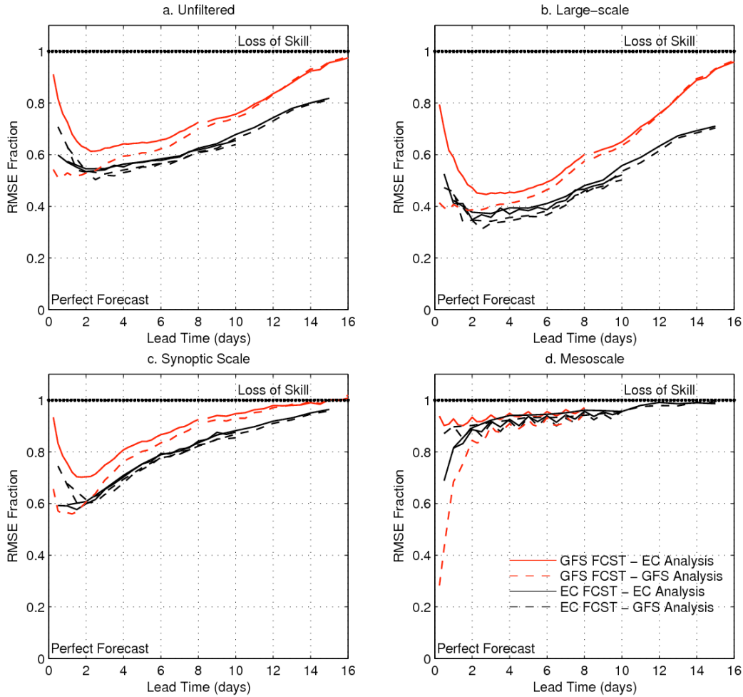
Figure 3. Root mean square error (RMSE) fraction (forecast error divided by persistence error) of zonal wind speed (U850) as a function of forecast lead time. (a) Unfiltered data, (b) large-scale filtered data, (c) synoptic scale filtered data, and (d) mesoscale filtered data. Black curves are for ECMWF and ECMWF-ctl. Red curves are for GFS. Solid curves are using ECMWF analysis to calculate errors while dashed curves use the GFS analysis. In (d), the GFS mesoscale filtered data for lead time longer than 8 days are not resolved because of low resolution. (Adapted from Kerns and Chen 2014b.)
