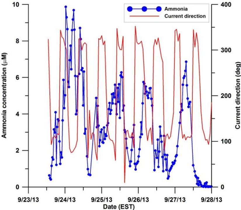
Figure 4. Ammonium concentrations are plotted with current direction.
