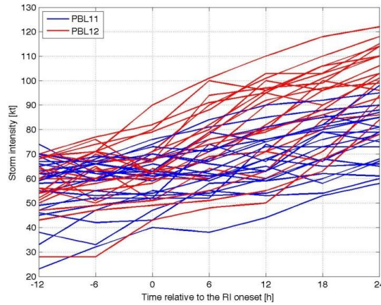
Figure 6: Plot of the storm intensity in kt for PBL11 (blue) and PBL12 (red) forecasts. Only forecasted RI events in PBL12 but not in PBL11 are shown.
