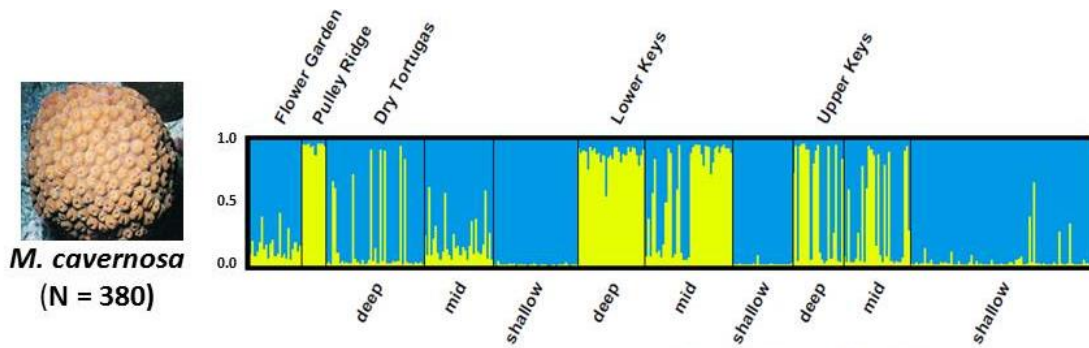
Figure 1: Results of STRUcTURE analysis of Montastraea cavernosa samples showing that Pulley Ridge samples belong to the same population as deep sites in the Florida Keys , whereas samples from the Flower Garden Banks belong to the same population as shallow sites in the Florida Keys.
