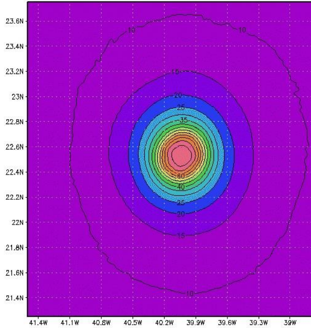
Figure 4: Surface pressure drop, \Delta p = p_{\infty} - p_{\min} for idealized TC; same time and domain as for Figure 3; where p_{\infty} = 1010.3 hPa. Contours every 5 hPa. The maximum \Delta p = 79.5 hPa ( p_{\min} = 930.8 hPa absolute). Radius of 10 hPa contour \sim 120 km. At model level one ( z \sim 25 m) this radius is \sim 275 km – see Figure 5.
