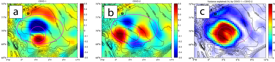
Figure 9. Spatial patterns of CSVD-1 (a) and CSVD-2 (b), shown as correlation maps; variance explained by SSH reconstructed with CSVD-1 and CSVD-2 (c). Two ellipsoidal contours, along which the wavenumber-frequency spectra are computed, are shown.
