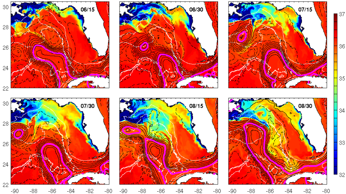
Figure 1: Sea surface salinity (colors, SSS) extracted from the assimilative 1/50^\circ model simulation (zoom over the eastern GoM), from June 15 to August 30, 2014. In black contours is the Sea Surface Height (SSH) every 6 cm. Positive SSH with respect to the basin mean is in continuous lines, negative SSH is in dashed lines. The Loop Current is in magenta (SSH value of 17 cm over the basin mean, as defined by Leben, 2005). The white lines indicate the isobaths 200, 2000 and 3000 m.
