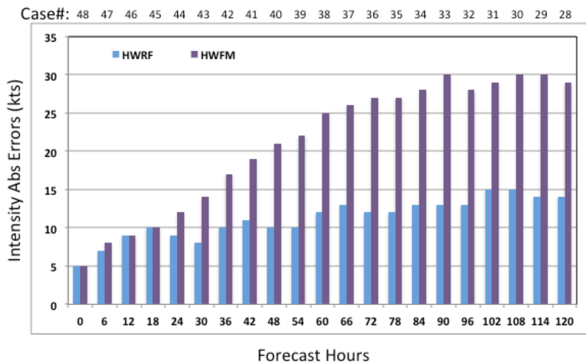
Figure 2. Track and intensity forecast verification of Hurricane Leslie. (a). Track; (b). Intensity.
