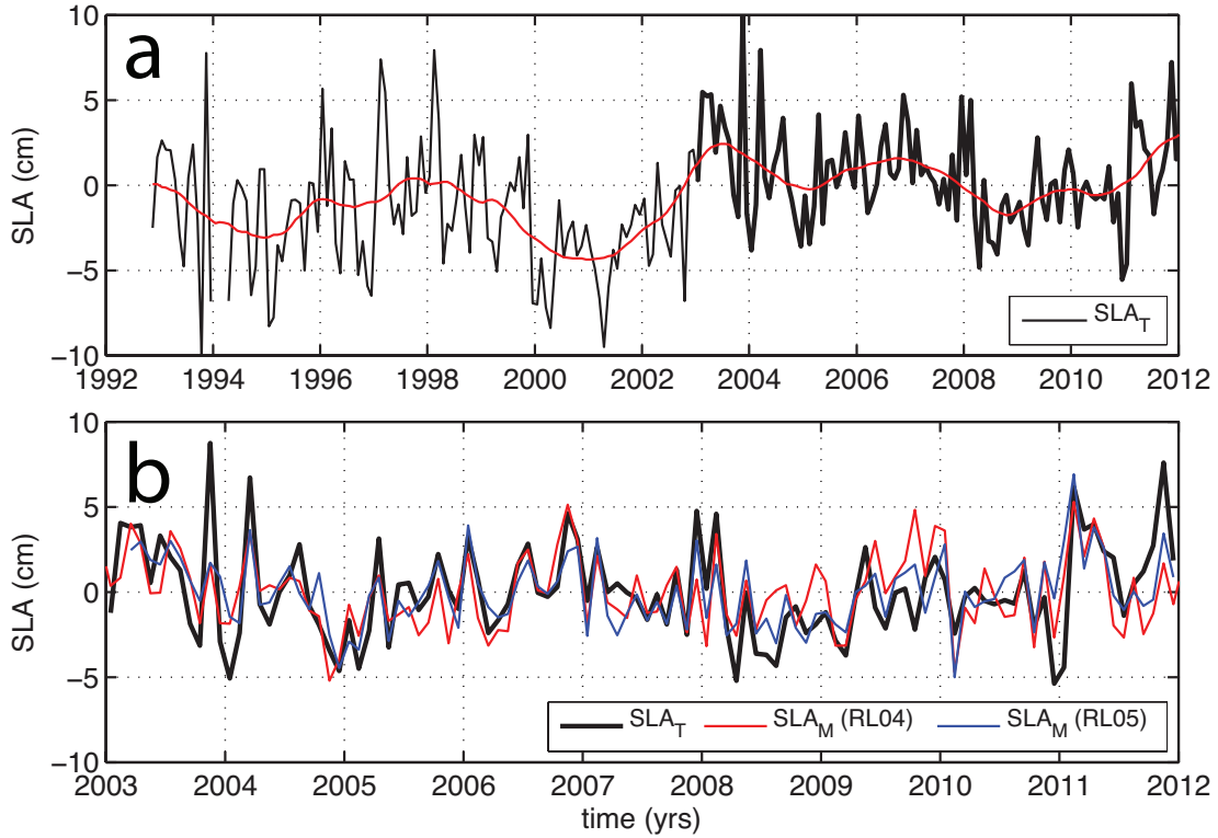
Figure 11. (a) The non-seasonal SLA_T from satellite altimetry for the 1992-2011 time period (black) and its yearly running mean (red); (b) the de-trended time series of the non-seasonal SLA_T (black) versus SLA_M from GRACE RL04 (red) and RL05 (blue) products for the 2003-2011 time period. The time series are averaged over 25^\circ W - 45^\circ W and 73^\circ N - 77^\circ N .
