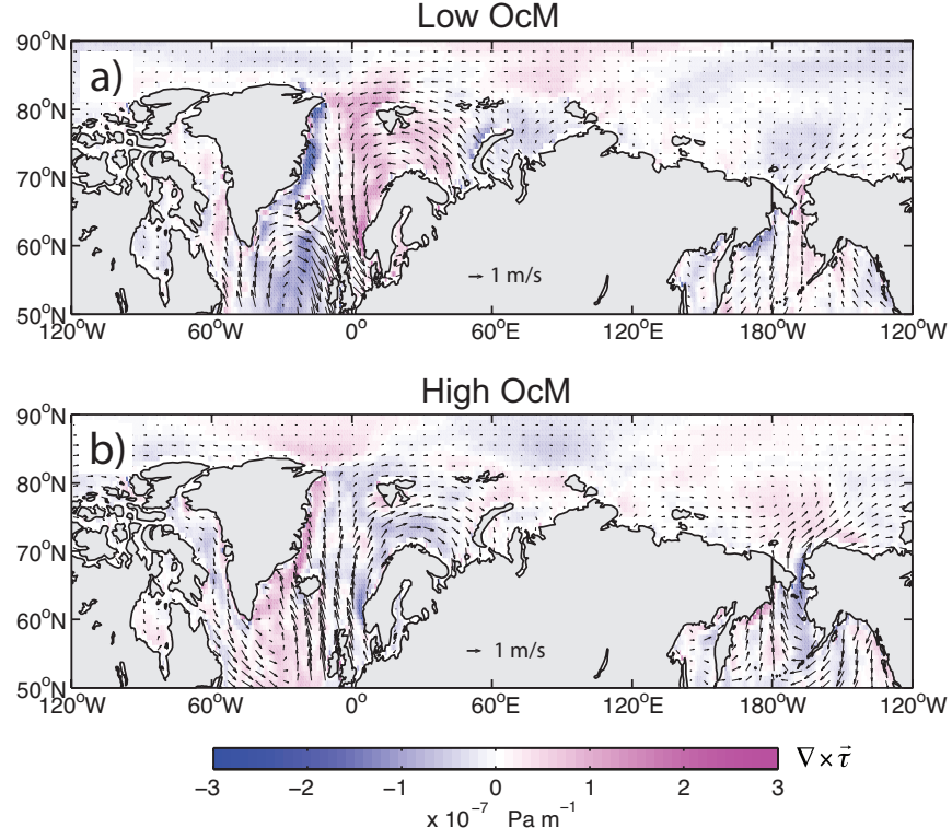
Figure 22. The 10 m height wind vectors and wind stress curl (color) averaged over the period of low (a) and high (b) OcM anomaly, i.e. when OcM in Figure 2 is less than -1 cm and greater than 1 cm, respectively.
